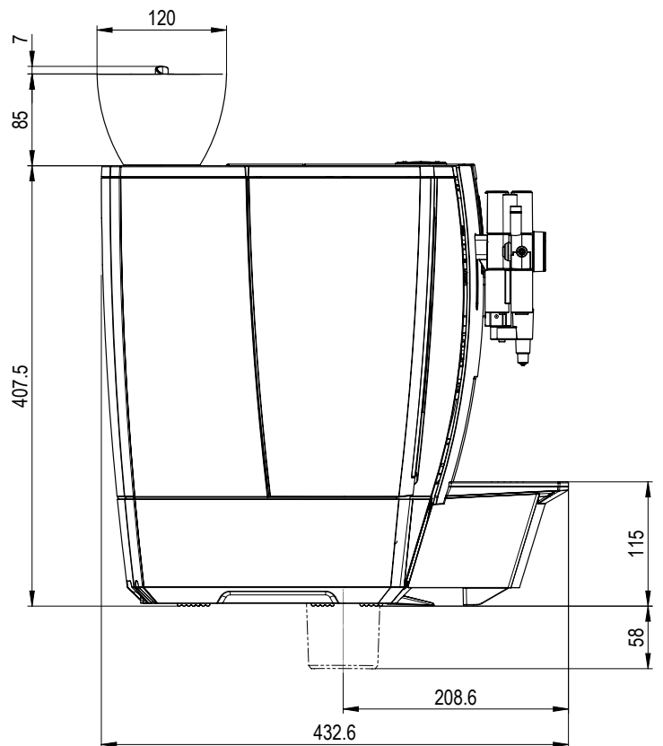
Side outline
